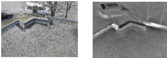
Figure 3: Convection heat loss at wall corner/flat roof perimeter detail. Masonry brick wall appears to be wet, due to moist warm interior air ex-filtrating through exterior wall system.
